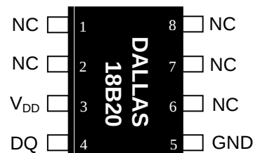
8-pin 150-mil SOIC (DS18B20Z)
