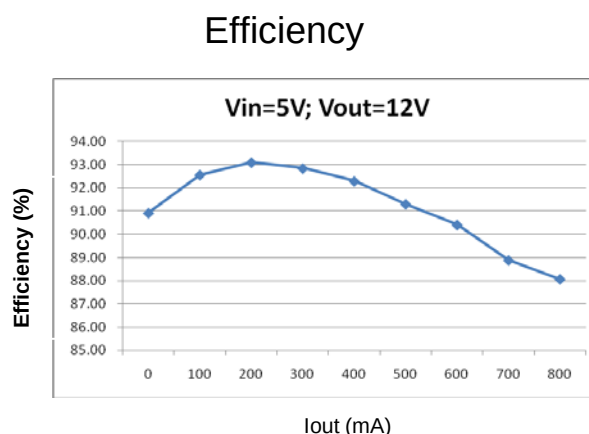
Figure 2. Efficiency Curve
