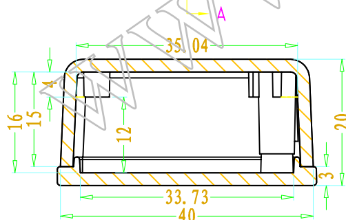
SEC B-B
