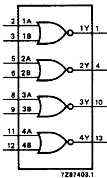
Fig.4 Functional diagram.
