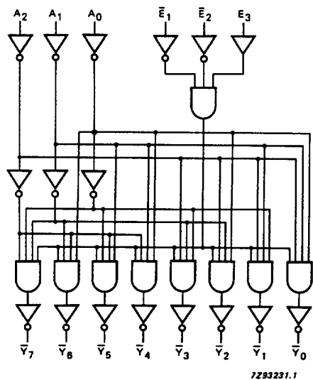
Fig.5 Logic diagram.
