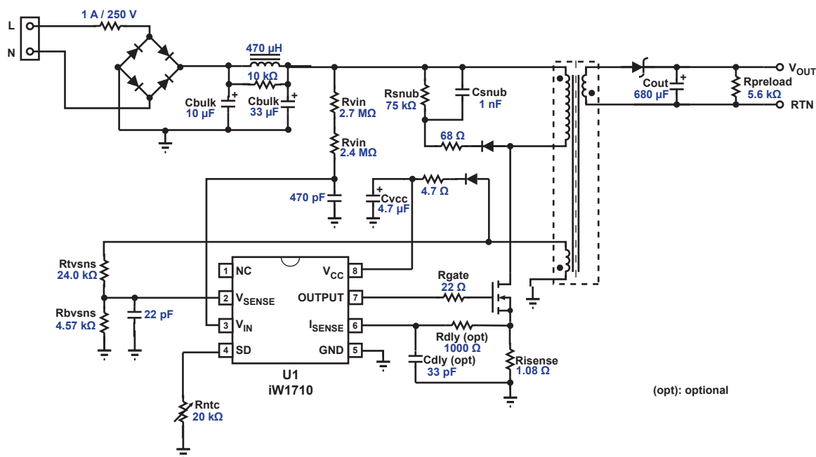
Figure 12.1 : Typical Application Circuit
