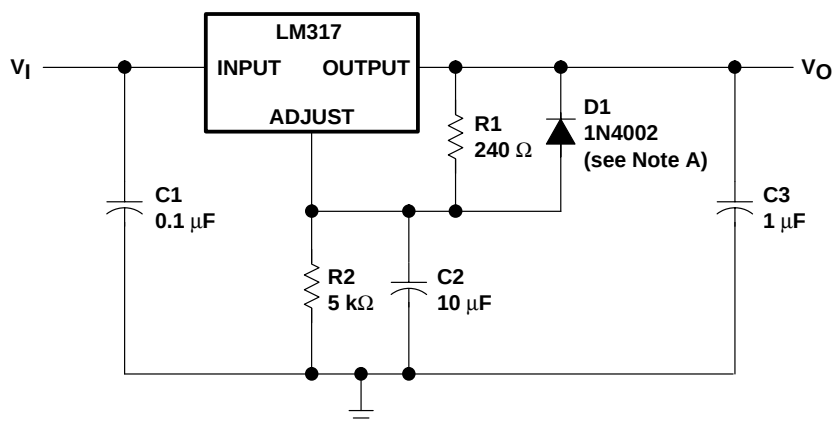
Figure 2. 0-V to 30-V Regulator Circuit
