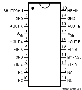
Top View Order Number LM4863MT See NS Package Number MTC20 for TSSOP
