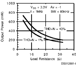
Output Power vs Load Resistance
