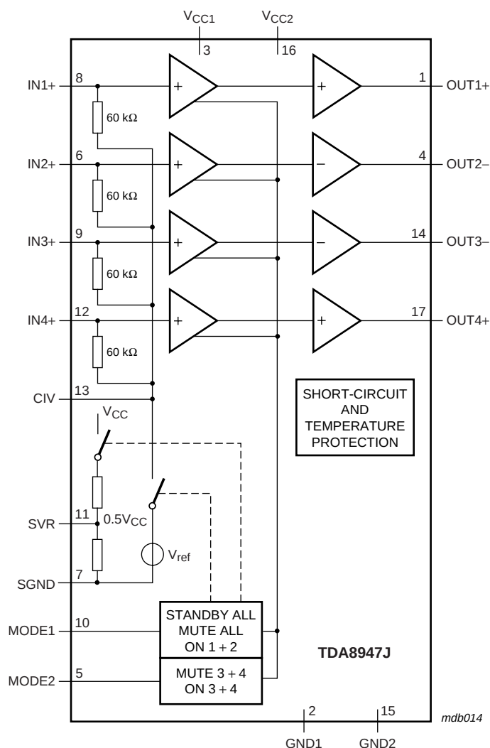
Fig 1. Block diagram
