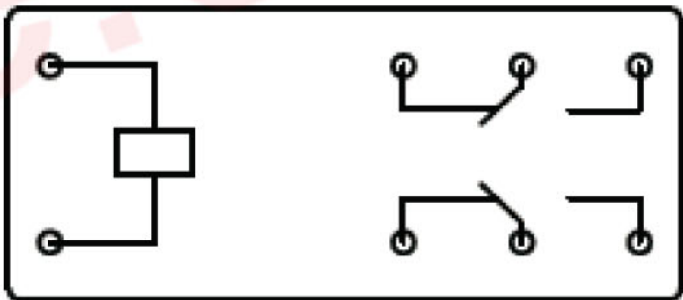
Conversion 2C type
