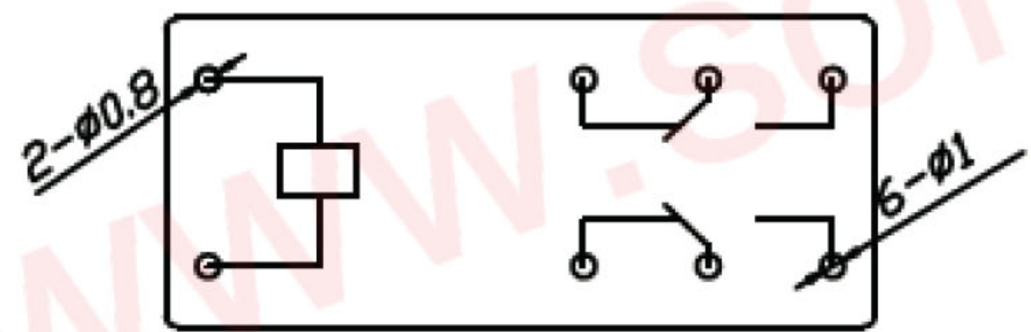
Electrical Diagram
