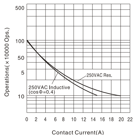
Endurance Curve
