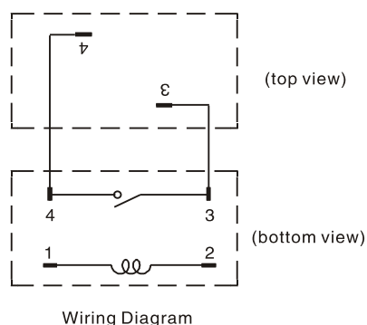
Wiring Diagram
