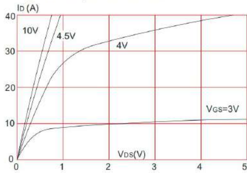
Figure 1: Output Characteristics
