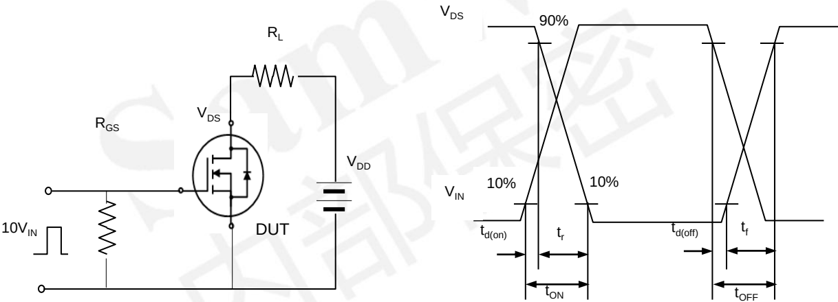
Fig. 16. Switching time test circuit & waveform
