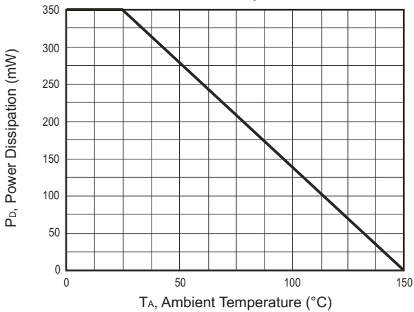
Fig.8 Power Dissipation vs. Ambient Temperature
