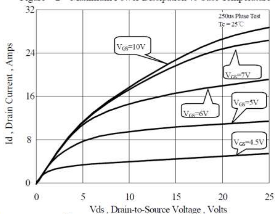
Figure 4 Typical Output Characteristics
