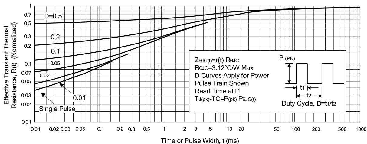
Fig.4 Thermal Response
