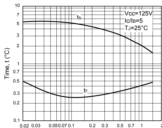
Fig.3 Turn-Off Time
