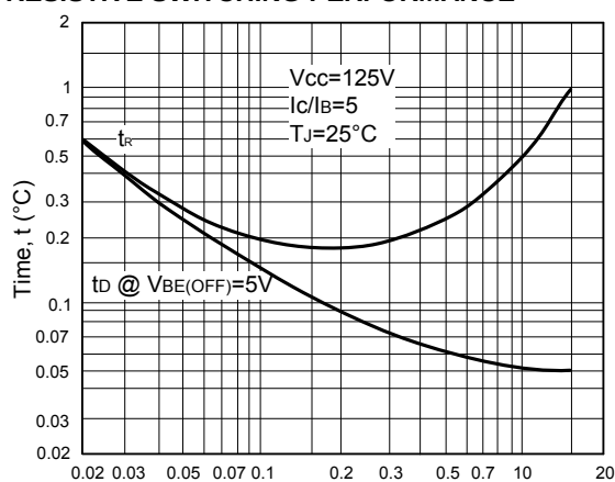
Fig.2 Turn-On Time
