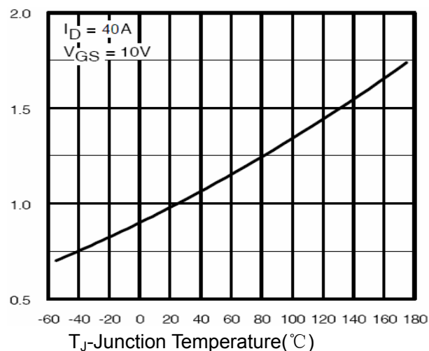
Figure 4 Rdson-Junction Temperature
