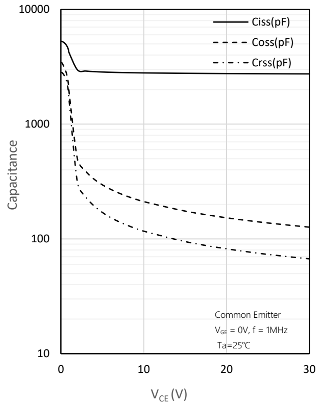
Fig. 10 Capacitance characteristics
