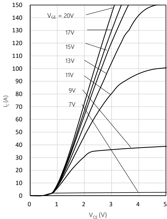
Fig. 3 Output characteristics
